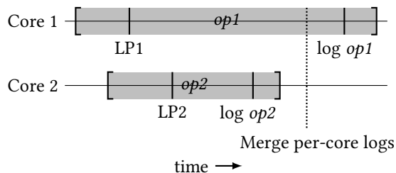
Figure 3: Two concurrent operations, op1 and op2 , running on cores 1 and 2 respectively. The grayed-out box denotes the start and end time of an operation. LP denotes the linearization point of each operation. “log” denotes the time at which each operation is inserted into that core’s log. The dotted line indicates the time at which the per-core logs are merged.
